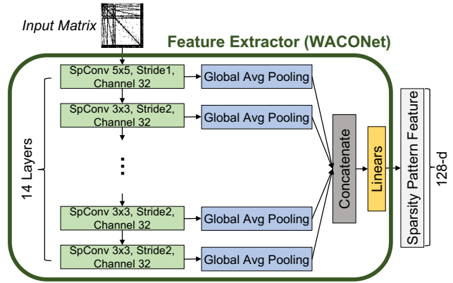
Figure 9: Network architecture of WACONet. We omitted non-linear activation layers in the figure.
