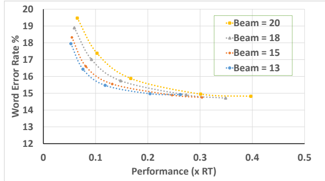
Fig. 4. Performance vs WER curve.
